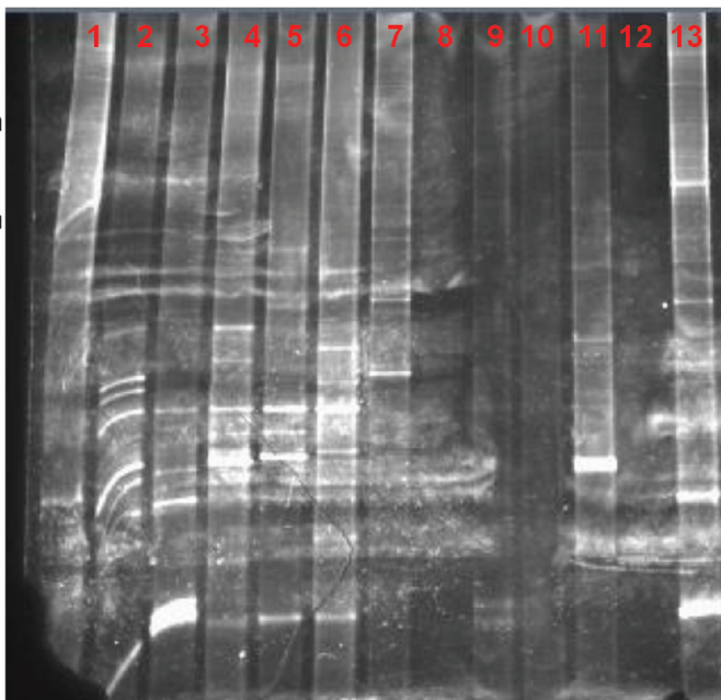
Figure 6. DGGE profiles of environmental bacterial aerosols (control and treated by plasma) and total aerosolized B. subtilis and P. fluorescens (culturable and nonculturable); bacterial colony forming units used were pooled from at least three repeats for each of the environments tested.
