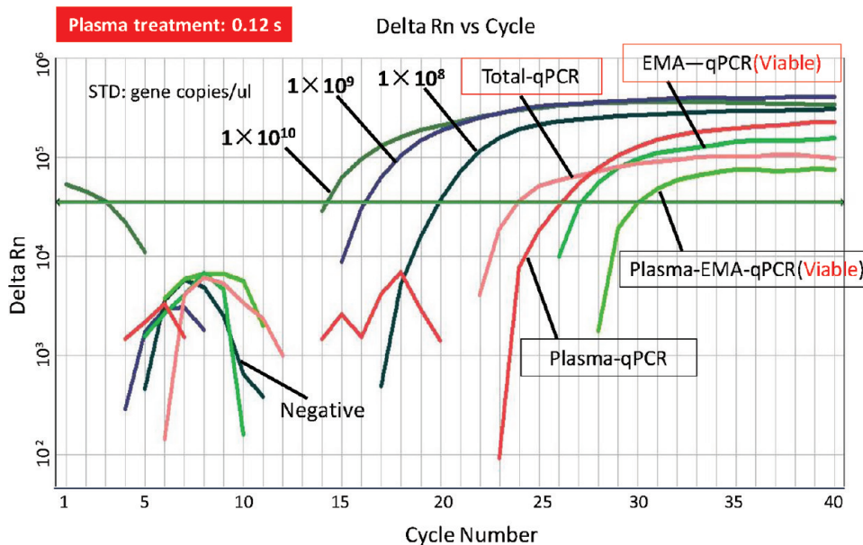
Figure 3. Total and viable fractions of airborne B. subtilis aerosol samples collected using the BioSampler with and without plasma treatment; Total-qPCR indicates the total B. subtilis concentration; EMA-qPCR (viable) indicates the total viable B. subtilis concentration without plasma treatment; Plasma-qPCR indicates the total B. subtilis concentration after the plasma treatment; Plasma-EMA-qPCR indicates the total viable B. subtilis concentration after the plasma treatment.
