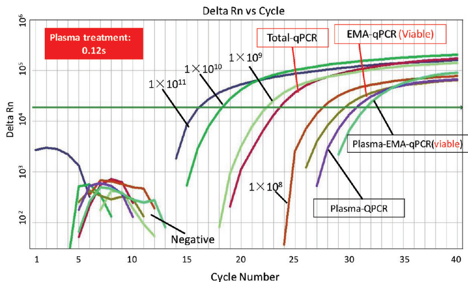
Figure 4. Total and viable fractions of airborne P. fluorescens aerosol samples collected using the BioSampler with and without plasma treatment; Total-qPCR indicates the total P. fluorescens concentration; EMA-qPCR (viable) indicates the total viable P. fluorescens concentration without plasma treatment; Plasma-qPCR indicates the total P. fluorescens concentration after the plasma treatment; Plasma-EMA-qPCR indicates the total viable P. fluorescens concentration after the plasma treatment.
